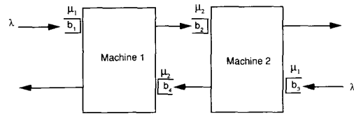
Fig. 8. The Rybko–Stolyar example of Section XIII.
